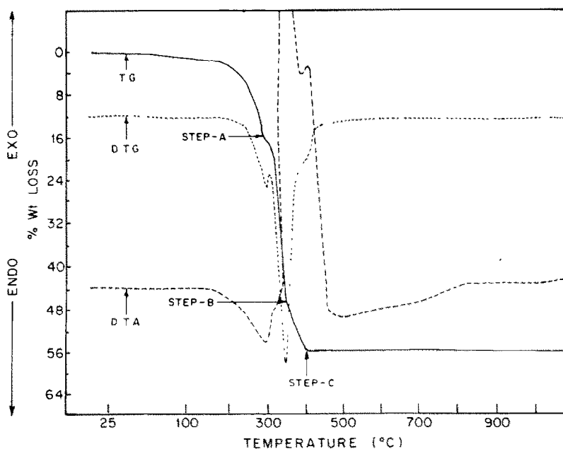
Fig. 1. TG, DTG and DTA curves of zinc citrate in air.
