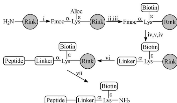
Scheme 3. Synthetic route for solid-phase peptide biotinylation. Reagents and conditions: (i) 2 equiv of Fmoc-Lys(Alloc)-OH, 2 equiv of benzotriazole-1-yl-oxy-tris-pyrrolidino-phosphonium hexafluorophosphate (PyBOP ® ) and 4 equiv of DIEA in DMF, rt, 1 h; (ii) 0.25 equiv of Pd(PPh 3 ) 4 , 24 equiv of PhSiH 3 in DCM, Ar, rt, 30 min×2; (iii) 2 equiv of biotin, 2 equiv of PyBOP ® and 4 equiv of DIEA in DMF, rt, 1 h; (iv) 20% piperidine in DMF, rt, 15 min×2; (v) 2 equiv of linker, 2 equiv of PyBOP ® and 4 equiv of DIEA in DMF, rt, 1 h; (vi) peptide synthesis; (vii) TFA/H 2 O/TIS (v/v/v 95:2.5:2.5).
