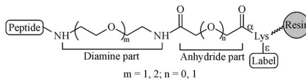
Scheme 1. Design of the linkers.
