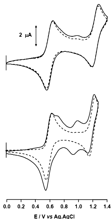
Figure 7. Cyclic voltammograms recorded in 0.10 M Bu 4 NPF 6 /CH 2 Cl 2 , scan rate 100 mV s -1 . Top 4MTZ , bottom 4ETZ ca. 10 -4 M. Dotted line: initial CV; solid line: after 5 h irradiation with 360 nm monochromatic light.
