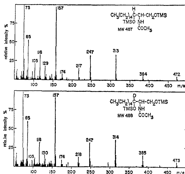
Figure 2. Mass spectra of 1,3-di-O-trimethylsilyl-N-acetyldihydrosphingosine (upper) and 1,3-di-O-trimethylsilyl-N-acetyldihydrosphingosine- \text{d}_3 (lower).
