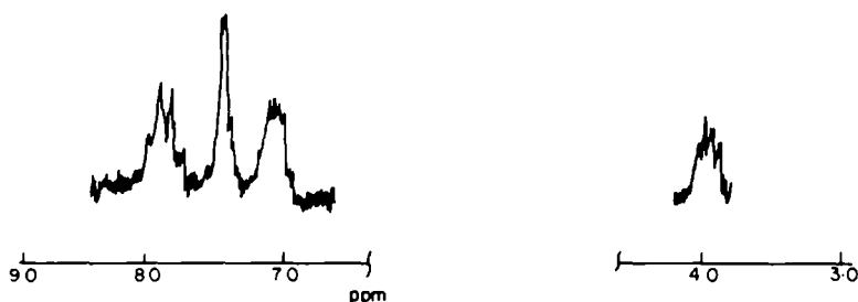
FIG 5. NMR spectrum of dioxyluciferin (VII) (DMSO- d_6 )
