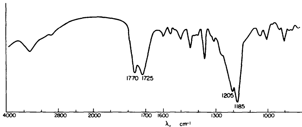
FIG 6. IR spectrum of dioxyluciferin diacetate (VIII) (KBr)
