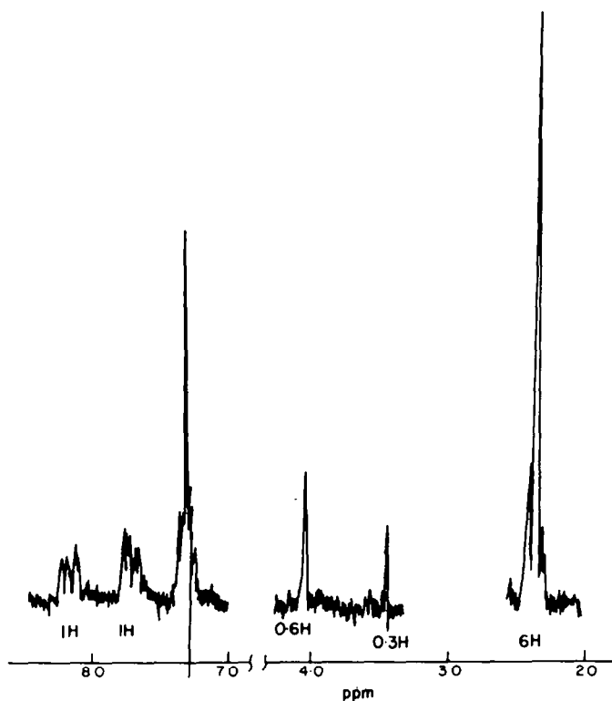
FIG 7. NMR spectrum of dioxyluciferin diacetate (VIII) ( \text{CDCl}_3 )
