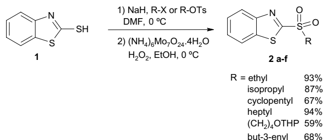
Scheme 1. Preparation of the benzothiazolyl sulfones.
