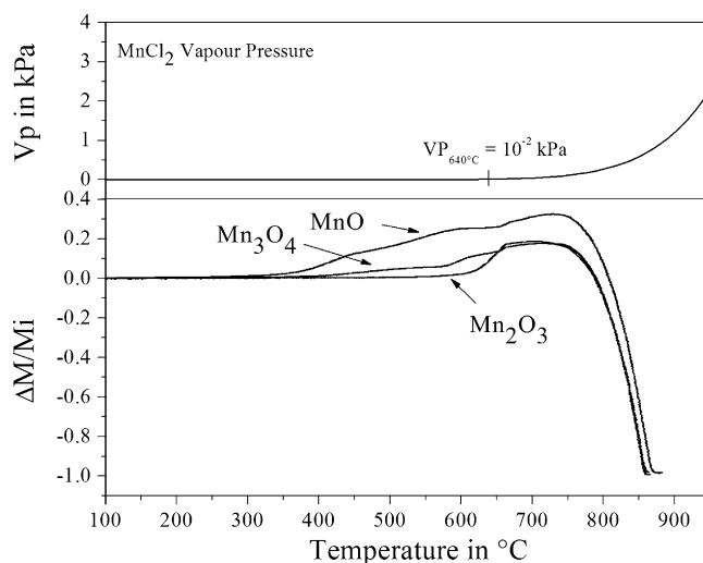
Fig. 3. Non-isothermal chlorination reactions of MnO, \text{Mn}_3\text{O}_4 and \text{Mn}_2\text{O}_3 .
