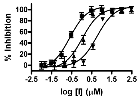
Figure 5. IC 50 analysis for 2-(2)-13 (▼), 3-(3)-13 (▲), and 3-(3)-27 (■).
