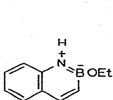
(I) \delta -29.7 ppm
