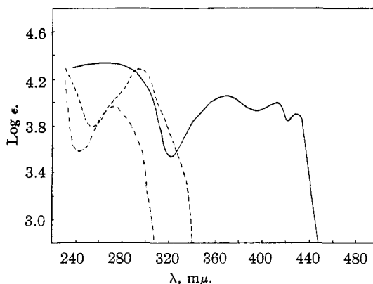
Fig. 1.—Ultraviolet absorption spectra of 1-skatyl-tetrahydroisoquinoline, VII (—); 1-(2'-carbethoxy-3'-indolylmethyl)-1,2,3,4-tetrahydroisoquinoline, IX (---); and XII (- - -) in ethanol.
