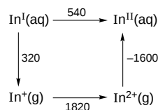
Scheme 1. Conversion of In I to In II ( \Delta G Values in kJ)
