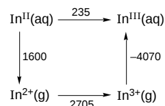
Scheme 2. Conversion of In II and In III ( \Delta G Values in kJ)
