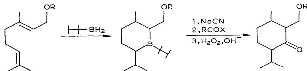
myrcene (I).
