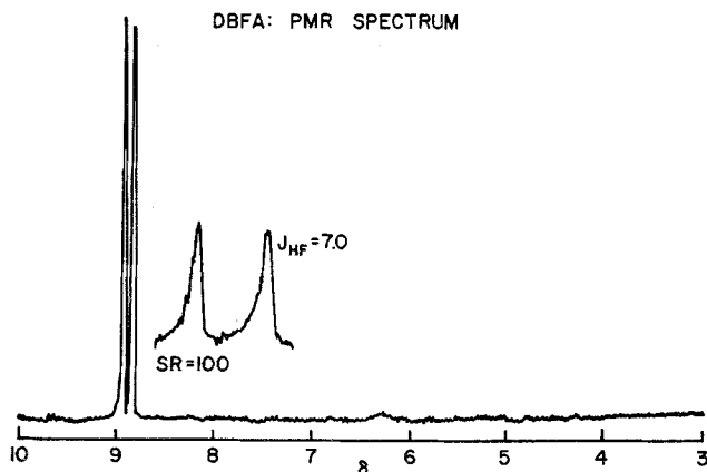
Fig. 2. ^1\text{H} NMR spectrum of DBFA
