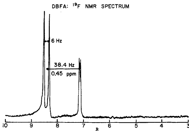
Fig. 3. ^{19}\text{F} NMR spectrum of DBFA
