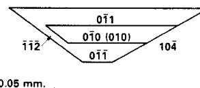
Distance between 010 and 0\bar{1}0 faces = 0.03 mm.
