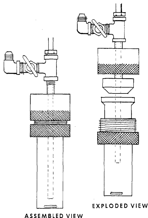
Figure 1.—Kel-F reactor.
