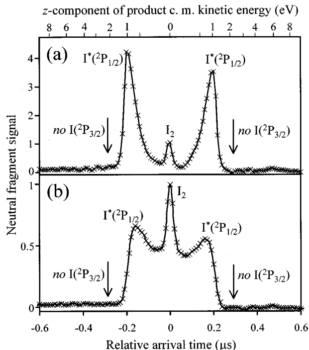
FIG. 3. Neutral photofragment TOF spectra obtained in 395 nm photodestruction of I_2^- with the laser polarization (a) parallel and (b) perpendicular to the flight axis ( z ). The fragment spatial distributions are truncated at the entrance into the reflectron (see Fig. 2). Top axis is the z -component of fragment c.m. translational energy.
