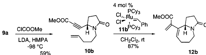
Scheme 6 Cyclization of Enynes Using Ruthenium Catalyst ( 11b )
