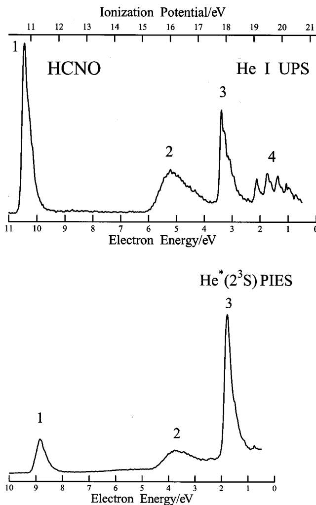
Figure 2. He I UPS and He*(2 3 S) PIES spectrum of HCNO.
