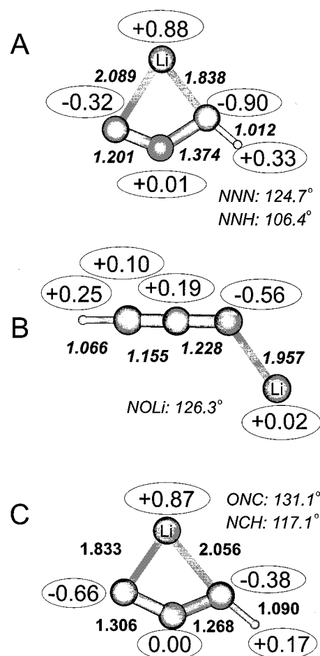
Figure 13. Calculated structure (distances in angstrom) and total atomic charges of HNNNLI (A), HCNOLI(I) (B), and HCNOLI(II) (C) radicals.
