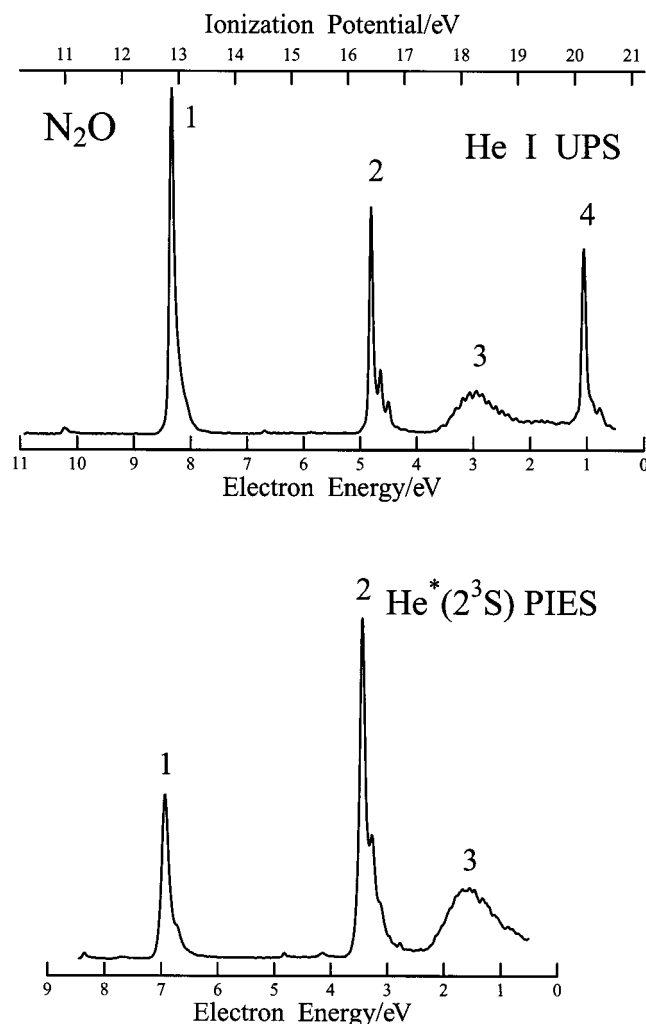
Figure 1. He I UPS and He*(2 3 S) PIES spectrum of NNO.
