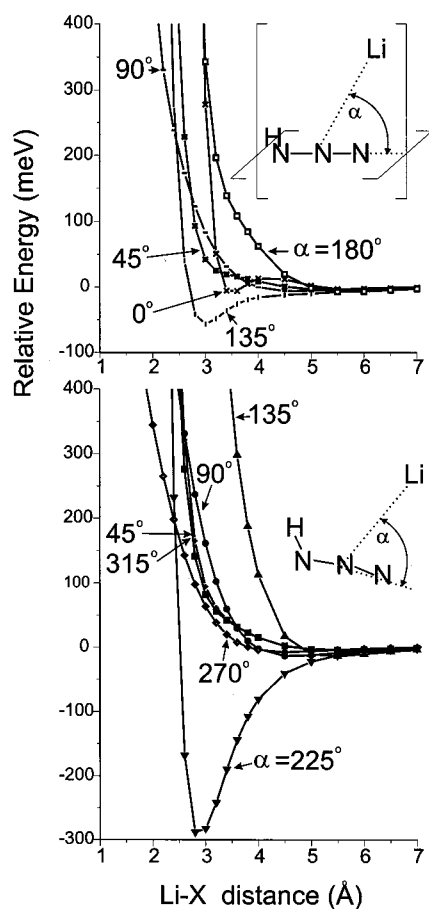
Figure 12. Calculated interaction potential curves between HNNN and Li( 2^2S ) as functions of distance between the Li atom and the center of mass of the molecule.
