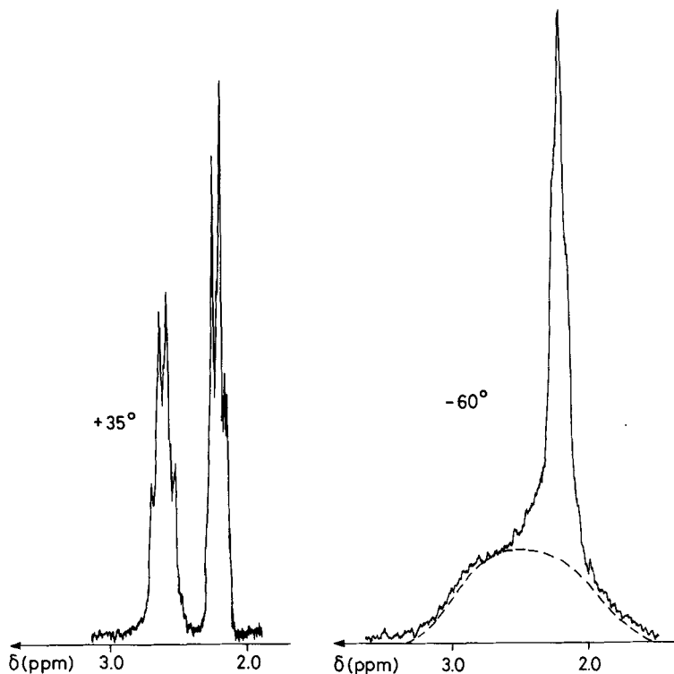
Fig. 2. T -Dependence in the ^1\text{H} -NMR. spectrum of the allylic hydrogen atoms of 3 centered at \delta 2.6 ppm
