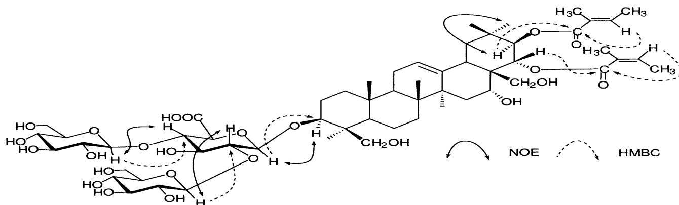
Chart 3. Some Key NOEs and Long-Range Correlations Observed in ROESY and HMBC Experiments of Compound 4
