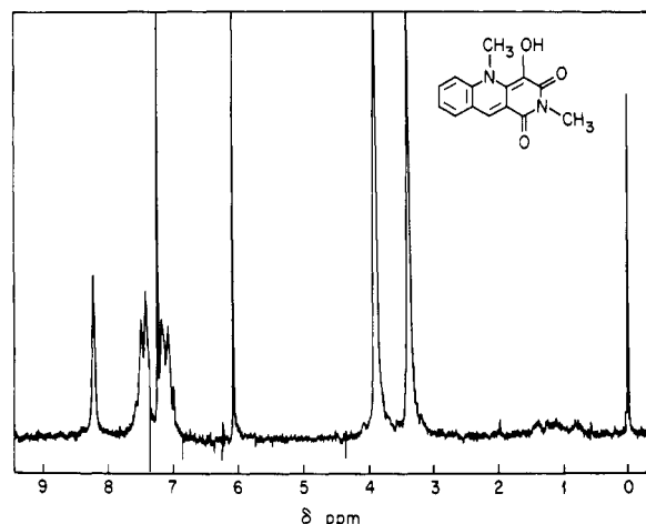
Figure 3. NMR spectrum of 3,10-dimethyl-1-hydroxy-1,5-dideazaizoxaloxazine (0.008 M in CDCl 3 , anaerobic). The peak at 6.03 ppm disappeared after the solution was shaken with D 2 O.
