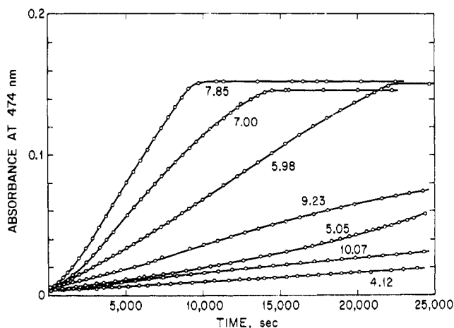
Figure 6. Plots of absorbance (474 nm) vs. time for the oxidation of dihydro-10-methyl-3-sulfo-1,5-dideazaisoalloxazine (IIIc-H 2 ) in oxygen-saturated buffers (pH 5–6, acetate; pH 6–8, phosphate; pH 9–10, carbonate) at 30 °C. [IIIc-H 2 ] = 1.7 \times 10^{-5} M. [O 2 ] \approx 8 \times 10^{-4} M. Numbers on the curves indicate the pH value.
