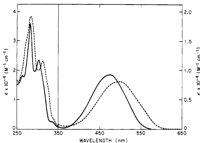
Figure 1. Absorption spectra of 3,10-dimethyl-1,5-dideazaisoalloxazine (III, solid line) and 8-cyano-3,10-dimethyl-1,5-dideazaisoalloxazine (IV, dashed line) at pH 7.0.
