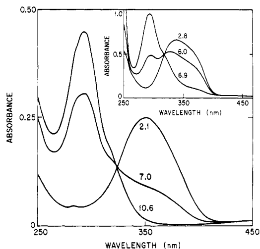
Figure 2. Absorption spectrum of dihydro-10-methyl-3-sulfopropyl-1,5-dideazaisoalloxazine ( 2 \times 10^{-5} M) and 8-cyanodihydro-10-methyl-3-sulfopropyl-1,5-dideazaisoalloxazine (inset, 4.8 \times 10^{-5} M) at three different pH values. Number on each curve indicates the pH value.
