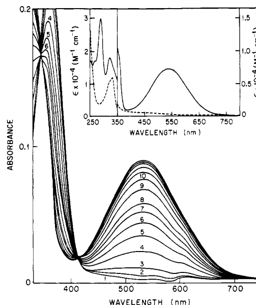
Figure 4. Formation of 3,10-dimethyl-1-hydroxy-1,5-dideazaalloxazine (IX) anaerobically from dihydro-3,10-dimethyl-5-hydroperoxy-1,5-dideazaalloxazine (VIII, 1.8 \times 10^{-5} M) at pH 8 (phosphate), 30 °C. Lines 1–3 were taken 15 min apart, lines 4–8 30 min apart, and lines 9 onwards were taken at 60-min intervals. Inset is the absorption spectrum of IX at pH 7 (phosphate). Dotted line was obtained after passing oxygen into the solution of IX for a few minutes.
