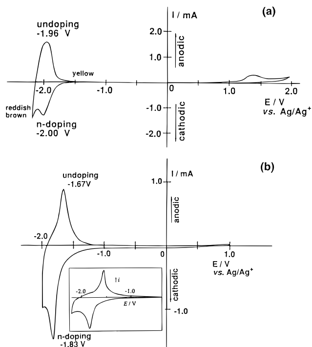
Figure 2. Cyclic voltammograms of films of (a) P(5,8-Qx) and (b) P(2,6-Qx) on platinum plates in a \text{CH}_3\text{CN} solution of [(\text{C}_2\text{H}_5)_4\text{N}]\text{ClO}_4 (0.1 M). The sweep rate is 10 \text{ mV s}^{-1} . Use of a \text{CH}_3\text{CN} solution of [(n\text{-C}_4\text{H}_9)_4\text{N}]\text{ClO}_4 for P(2,6-Qx) gives the CV curve shown in the inset in (b).
