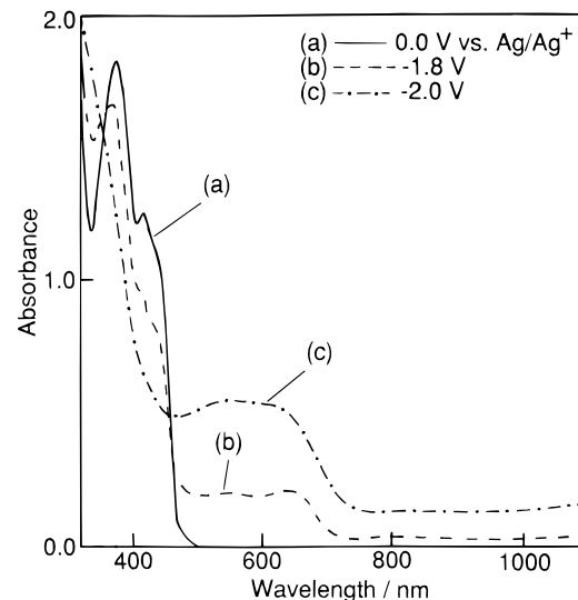
Figure 3. Changes in the absorption spectrum of a film of P(5,8-Qx-diPh) on an ITO electrode during electrochemical n-doping in a \text{CH}_3\text{CN} solution of [(\text{C}_2\text{H}_5)_4\text{N}]\text{ClO}_4 (0.1 M).
