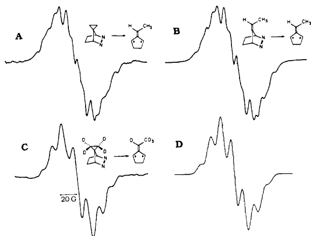
Figure 3. Hyperfine structure in \Delta m_s = 2 region of spectra for 2 and 17 and simulation for 17 .
