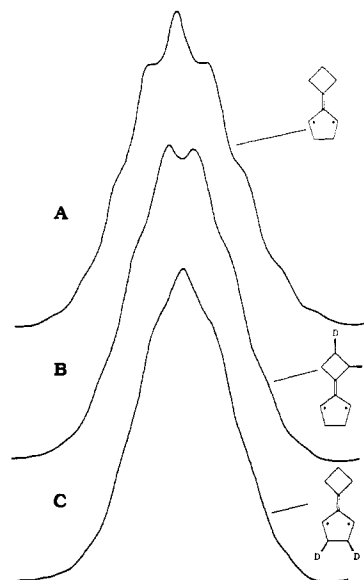
Figure 5. Absorption spectra, obtained by integration of analogous spectra from Figure 4, for \Delta m_s = 2 region of 9 , 14 , and 15 .
