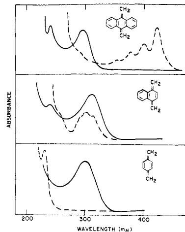
Figure 2. Uv spectra of the quinodimethanes at 77°K (—) and polymers formed on warming to 20°C (---). The quinodimethane and the polymer spectra are not reproduced on the same absorbance scale.
