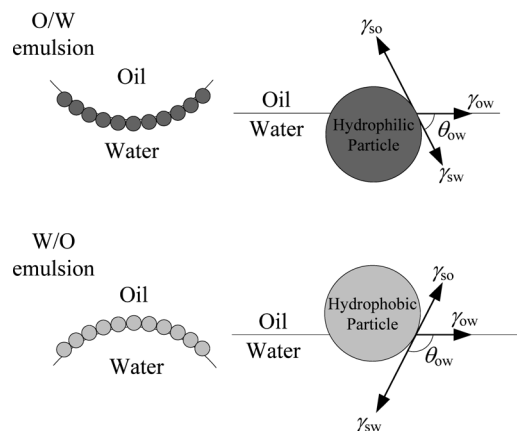
Fig. 3. Formation Mechanism of Pickering Emulsion
