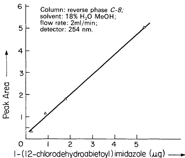
Fig. 1. Standard Curve in HPLC for 1-(12-Chlorodehydroabietoyl)imidazole (4). Column: reverse phase C-8; solvent: 18% H 2 O/MeOH; flow rate: 2 ml/min; detector: 254 nm.
