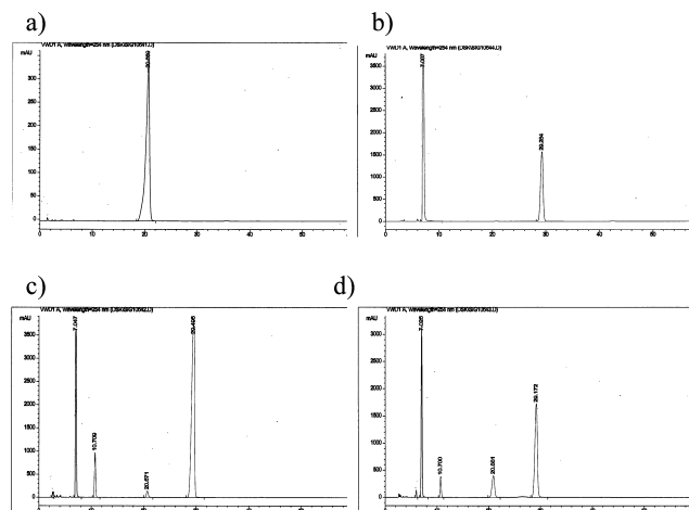
Figure 1. HPLC test results. The chromatograms were obtained using a Discovery HS C18, 5 \mu m; 25 cm \times 4.6 mm column with a flow rate of 1 mL/min; 70% methanol:30% water was used as eluant with a 10.0 \mu L injection. A UV detector was used at 254 nm. (a) Independently synthesized lactam; (b) reaction solution containing 1,2-diphenylhydrazine and tetrabutylammonium hexafluorophosphate prior to electrolysis; (c) reaction solution following the electrolysis; (d) co-injection of independently synthesized lactam and the electrolysis product solution.
