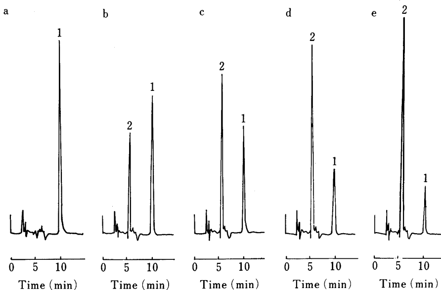
Fig. 1. Chromatograms of Sodium Sulbactam Degraded in 0.3 M Borate Buffer at pH 8.81, 35^\circ\text{C} and \mu=0.5
