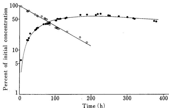
Fig. 2. Degradation Kinetics of Sodium Sulbactam (○) and II (●) during the Degradation of Sodium Sulbactam in HCl-KCl Buffer at pH 1.09, 35 °C and \mu=0.5
