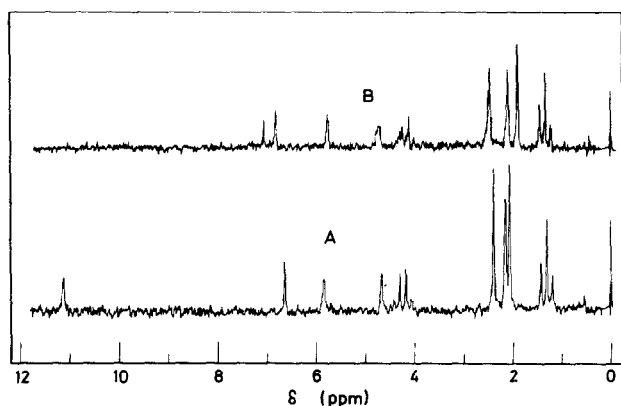
Figure 3. Nmr spectra of 1,19-dideoxy-8,12-dicarbethoxy-1,3,7,13,17,19-hexamethylbiladiene-ac in CCl 4 (A) and the corresponding nickel complex in CDCl 3 (B); TMS as an internal reference.
