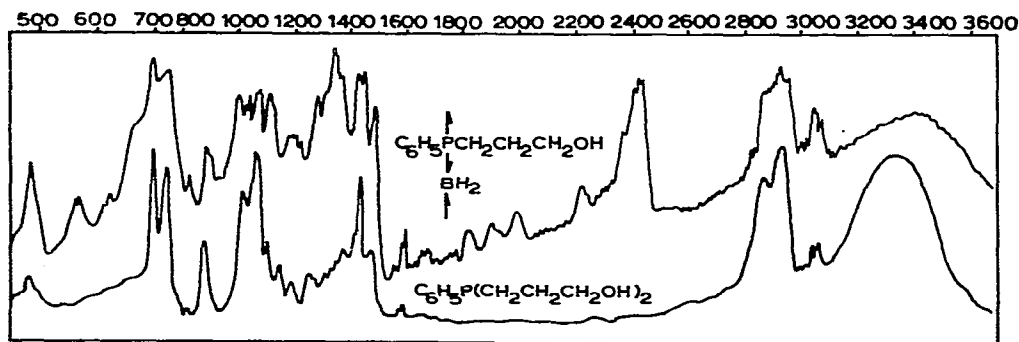
Fig. 6. Infrared spectra of polyphosphinoborane hydrolysis product (KBr pellet) and dioxypentylphenylphosphine (liquid).
