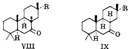
VIII IX a, R = \text{CH}_2\text{CHO} b, R = \text{CH}_2\text{CO}_2\text{H} c, R = \text{CH}_2\text{CO}_2\text{Me} d, R = (\text{CH}_2)_2\text{OH}
