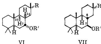
VI VII a, R = (\text{CH}_2)_2\text{OH} , R' = H b, R = (\text{CH}_2)_2\text{OAc} , R' = Ac
