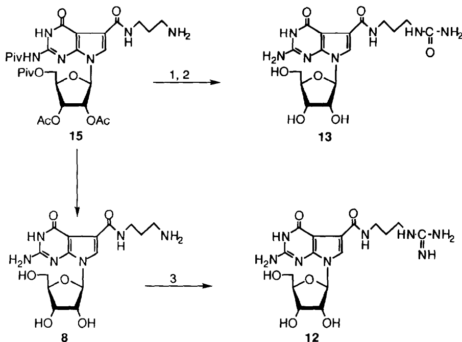
Scheme 3 Reagents and Conditions : 1) TMS-N=C=O, CH 2 Cl 2 , rt, 14 h; 2) NH 3 gas, MeOH, sealed tube, 70 °C, 72 h; 3) aminoiminomethanesulfonic acid, K 2 CO 3 , H 2 O, rt, 5h.
