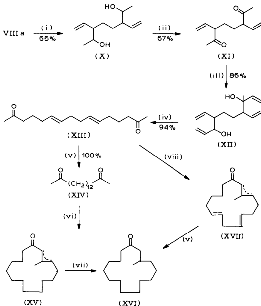
SCHEME 2. (i) \text{CH}_3\text{CHO} , \text{TiCl}_4 , \text{CH}_2\text{Cl}_2 , -78^\circ\text{C} . (ii) \text{CrO}_3 -3,5-dimethylpyrazole. (iii) \text{CH}_2=\text{CHMgCl} , THF. (iv) \text{KH} , THF, reflux. (v) \text{H}_2 , \text{Pd/C} , EtOH. (vi) and (vii) see ref. [12]. (viii) i\text{-Bu}_2\text{AlOPh} , pyridine, THF- n -hexane, reflux.
