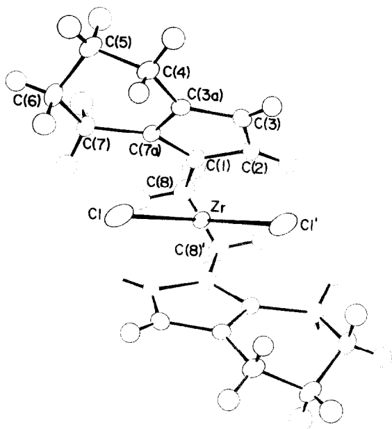
Fig. 1. Molecular structure of [ S,S ]-ethylenebis( \eta^5 -tetrahydroindenyl)zirconium dichloride ( 2 ).
