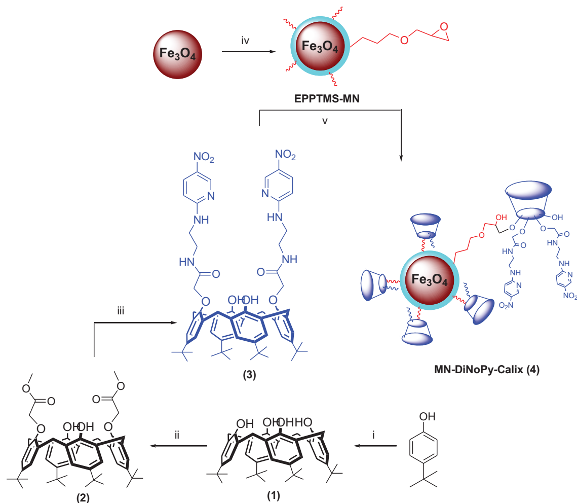
Scheme. Synthesis of MN-DiNoPy-Calix . Reaction conditions: i) \text{HCHO} , \text{NaOH} ; ii) methylbromoacetate, \text{K}_2\text{CO}_3 , \text{CH}_3\text{CN} ; iii) 2-(2-aminoethylamino)-5-nitropyridine, \text{CH}_2\text{Cl}_2/\text{CH}_3\text{OH} ; iv) 3-(2,3-epoxypropoxy)propyl]trimethoxysilane, tetraethyl orthosilicate, \text{NaF} , \text{H}_2\text{O} ; v) \text{NaH} , \text{THF}/\text{DMF} .
