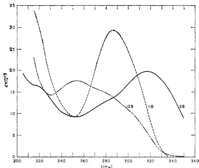
Fig. 2.—Ultraviolet absorption spectra of 2b and its interconversion products: — 2b in 0.1 N HCl; --- 12b from 2b in 0.1 N NaOH, spectra taken immediately; ---- 11b from 2b in 0.1 N NaOH, spectra after 22 hr.
