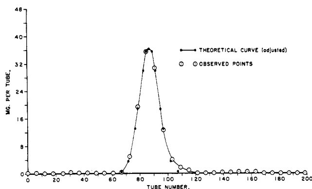
Fig. 1.—Countercurrent distribution of celesticetin.
