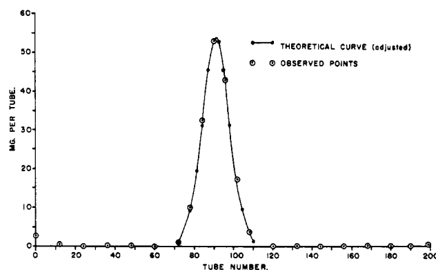
Fig. 2.—Countercurrent distribution of desalicytin.
