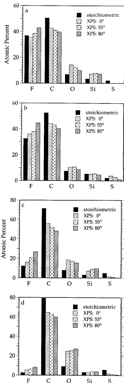
Figure 5. Angular-dependent XPS compositional analysis for polymer ultrathin films of siloxane terpolymers assembled on gold substrates as a function of side chain composition: (a) 70% perfluorocarbon, 30% alkyl disulfide side chains; (b) 41% perfluorocarbon, 21% alkyl disulfide side chains; (c) 23% perfluorocarbon, 77% alkyl disulfide side chains; (d) 5% perfluorocarbon, 95% alkyl disulfide side chains.
