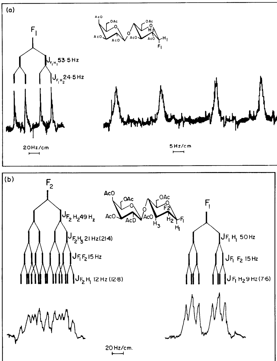
Fig. 2 . ^{19}\text{F} -Magnetic resonance spectra of hepta-O-acetyl lactosyl- \alpha -fluoride (III) (spectrum a ) and its 2-deoxy-2-fluoro derivative (VIII) (spectrum b ). Measurements were made in \text{CDCl}_3 at 87.4 MHz at 33^\circ with \text{CFCl}_3 as reference.
