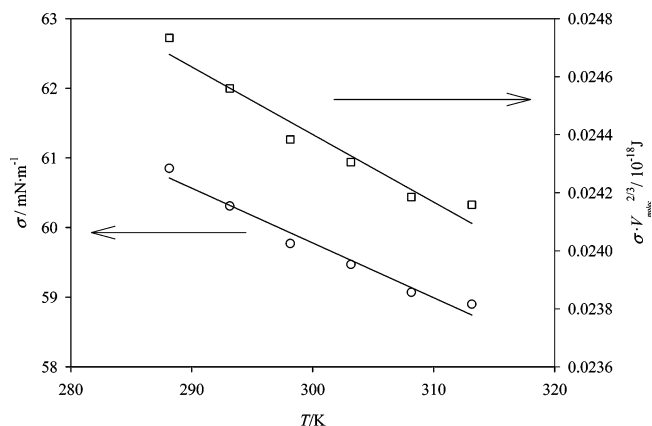
Figure 5. Plot of experimental values of surface tension \sigma (○) and \sigma \cdot V_{\text{molec}}^{2/3} (□) against T and fitted curves for [MMIM][MeSO 4 ].
