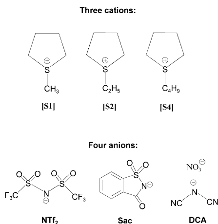
Scheme 1. Structures and abbreviations of the cations and anions employed in this work.
