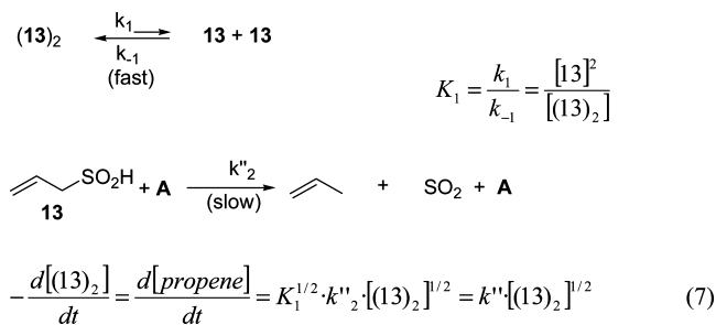
Scheme 12. Mechanism of the Desulfinylation in the Presence of Additive SO 2 or CF 3 CO 2 H
