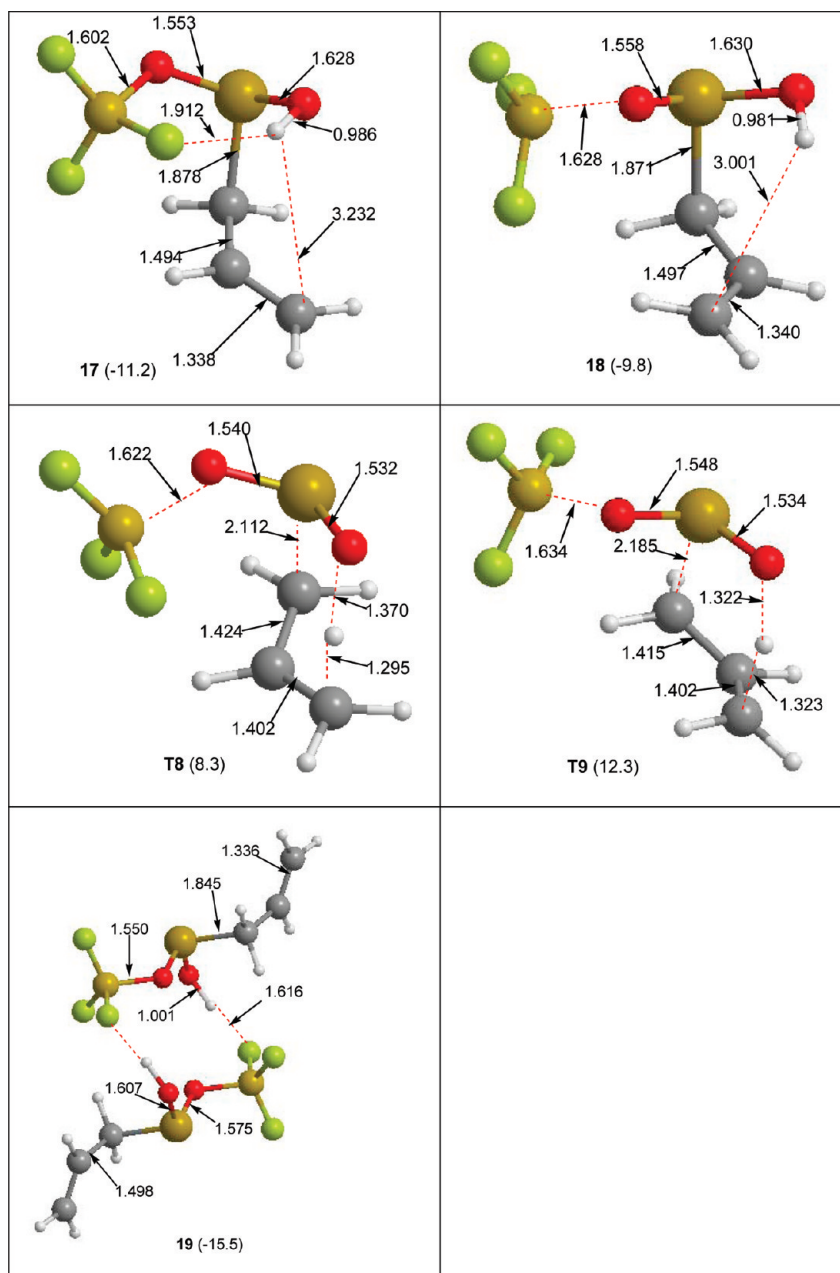
Figure 5. B3LYP/6-31+G(d,p) structures of the species located on the PES of the retro-ene reaction of 13 in the presence of \text{BF}_3 . Some selected bond distances are given in Å. CCSD(T)/6-311+G(d,p)//B3LYP/6-31+G(d,p) Gibbs free energy differences, including solvent effects, with respect to 0.5 \cdot (\mathbf{13})_2 (Table 3).
