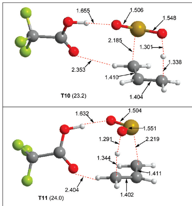
Figure 6. B3LYP/6-31+G(d,p) transition structures located on the PES of the retro-ene reaction of 13 in the presence of one molecule of CF 3 COOH. Some selected bond distances are given in Å. CCSD(T)/6-311+G(d,p)//B3LYP/6-31+G(d,p) Gibbs free energy differences, including solvent effects, with respect to 0.5•( 13 ) 2 (Table 3).
