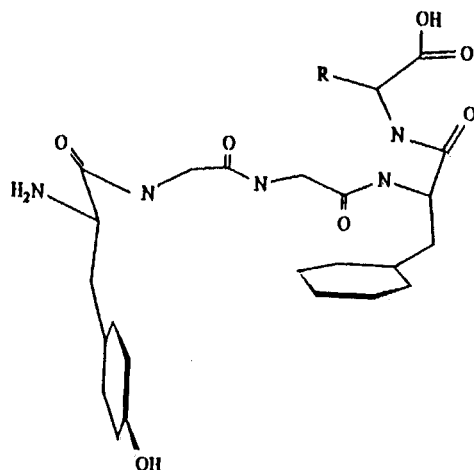
Figure 1. The geometry of NTI (A) and a possible receptor-bound conformation of enkephalin (B) at the \delta receptor.
