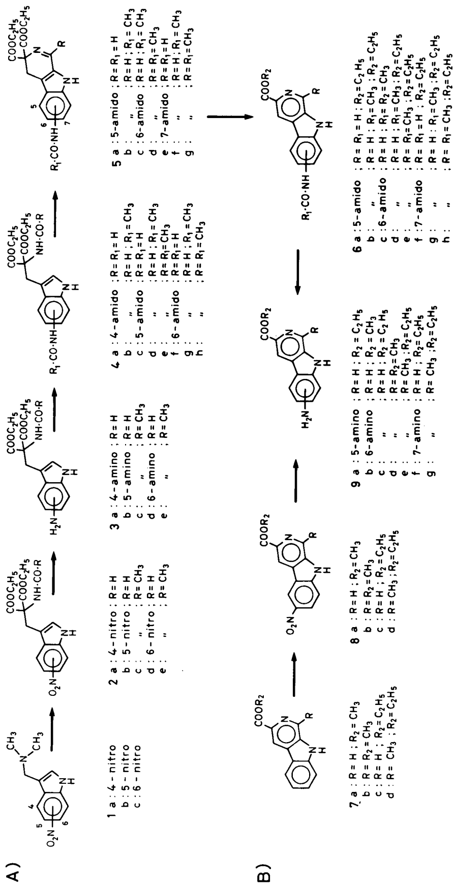
SCHEME 1
