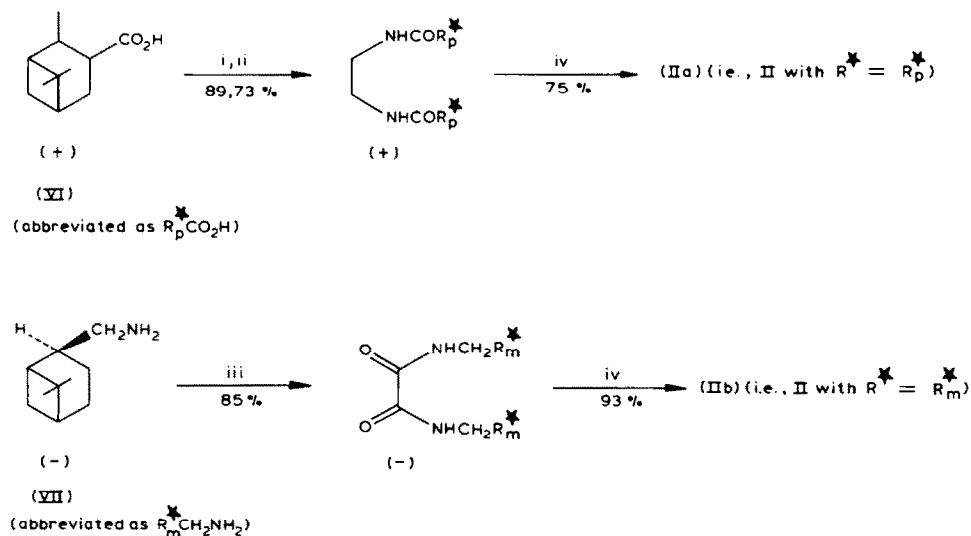
SCHEME 2. Reagents: i, \text{SOCl}_2 , reflux; ii, \text{H}_2\text{NCH}_2\text{CH}_2\text{NH}_2 , \text{NC}_3\text{H}_5 , 0^\circ\text{C} ; iii, (\text{CO}_2\text{Et})_2 , 20^\circ\text{C} , 2 h; iv, cf., iii and iv in Scheme 1.
