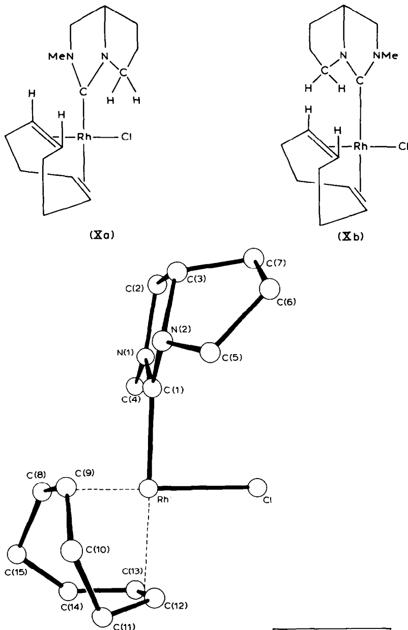
Fig. 1. The molecular structure of cis -[RhCl(COD) {(S)-CN(CH 2 CH 2 CH 2 )CHCH 2 NMe}], (Xa). Bond lengths: Rh—Cl 2.368(2), Rh—C(1) 2.004(4), Rh—C(8) 2.118(7), Rh—C(9) 2.101(8), Rh—C(12) 2.227(6), Rh—C(13) 2.206(5) Å; bond angle: Cl—Rh—C(1) 87.5(3)°.
