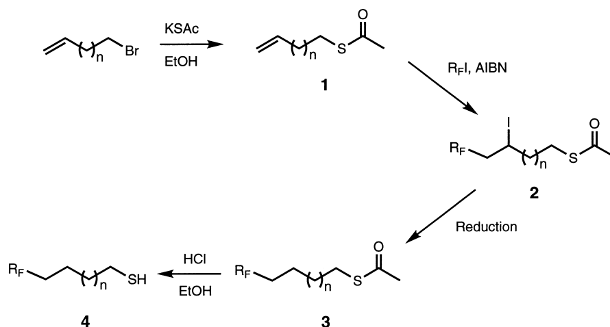
Scheme 1. Synthesis of terminally perfluorinated alkanethiols via radical addition of R_F-I to \omega -alkenyl thioacetates (method A).
