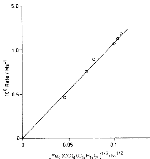
Fig. 8. Initial rate of formation of \text{Fe}(\text{CO})_2\text{Cl}(\eta^5\text{-C}_5\text{H}_5) vs. [\text{I}]^{1/2} .
