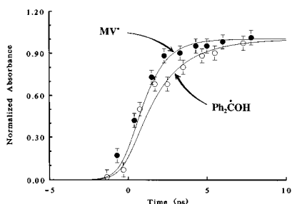
Figure 2. Kinetic (fs/ps) traces of the formation of MV^\bullet (●) and \text{Ph}_2\text{C(OH)}^\bullet (○) monitored at 605 and 530 nm, respectively. The smooth curves represent (a) the rise of MV^\bullet simulated by taking into account the instrumental response time of 700 fs (fwhm, see footnote 17a) and (b) the rise of \text{Ph}_2\text{C(OH)}^\bullet simulated by the convolution of the instrumental response time and the decarboxylation rate constant of k_{CC} = 8 \times 10^{11} \text{ s}^{-1} (see footnote 17b). The error bars reflect an uncertainty of \pm 0.005 absorbance units in the spectroscopic measurements.
