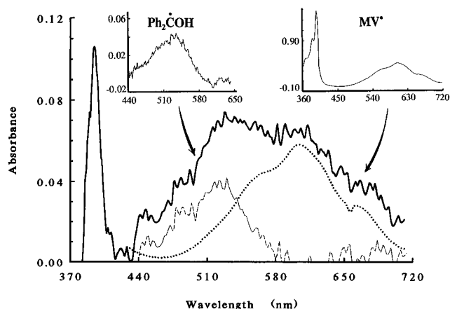
Figure 1. Transient absorption spectrum obtained at 1.0 ps following the 375-nm charge-transfer excitation of the [MV^+, \text{benzilate}^-] salt in water at 25 °C. Inset: (left) Authentic spectrum of the ketyl radical ( \text{Ph}_2\text{C(OH)}^\bullet ) in ref 16 and (right) the spectrum of reduced methylviologen ( MV^\bullet ) in ref 13c. Digital deconvolution of the broad absorption band (440–740 nm) in the experimental spectrum is shown as the composite of the spectra of \text{Ph}_2\text{C(OH)}^\bullet (—) and MV^\bullet (---), as described in footnote 15.
