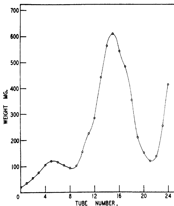
Fig. 1.—Craig countercurrent distribution curve for active concentrate of Veratrum viride showing peaks due to germitrine (tube 5) and neogermitrine (tube 15).
