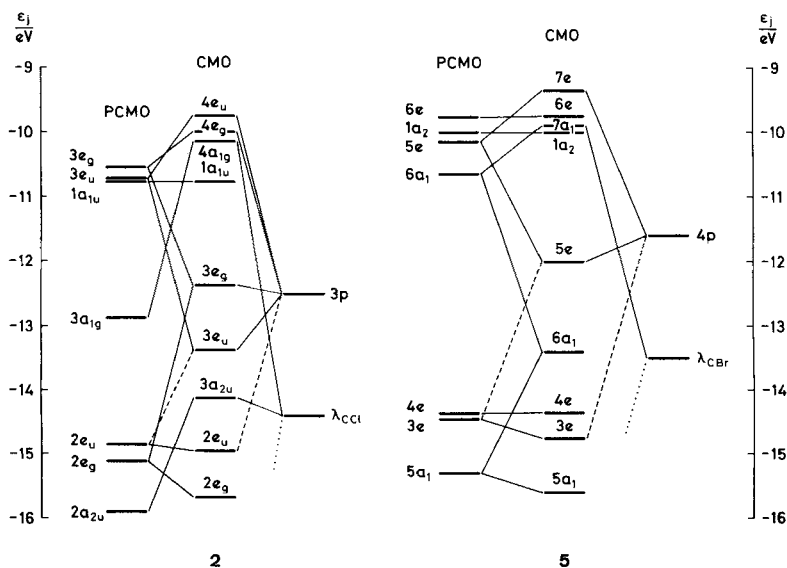
Fig. 3. Orbital correlation diagrams for 2 and 5 . PCMO = precanonical orbitals of the cubane moieties of 2 and 5 ; 3p = lone-pair orbitals of the pair of Cl atoms in 2 ; 4p = lone-pair orbitals of the Br-atom in 5 ; \lambda_{\text{CCl}} and \lambda_{\text{CBr}} = LMOs of the C–Cl \sigma -bonds in 2 and of the C–Br \sigma -bond in 5 .
